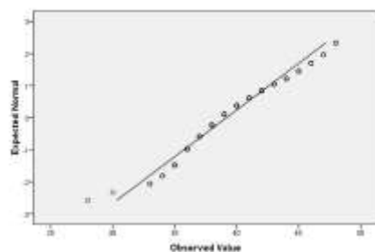
Normal Q-Q Plot of HASIL BELAJAR
